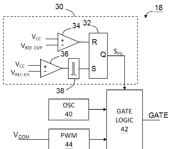
FIG. 2 (PRIOR ART)
