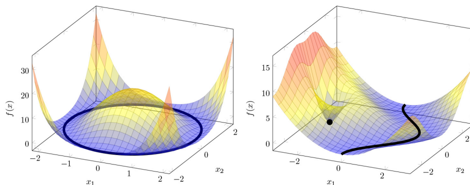
FIG. 5. Examples of functions f which satisfy the global NHC, with submanifolds \mathcal{Z} of zeros corresponding to the first and last submanifolds presented in Figure 2.
