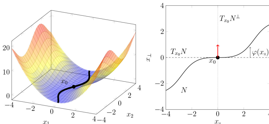
FIG. 4. Local view of the function around a minimum lying on a 1-dimensional manifold. Left: function around the minimum x_0 . Right: decomposition of \mathbb{R}^2 at x_0 between tangent space and normal tangent space T_{x_0}N + T_{x_0}N^\perp , and positive eigenvector of the Hessian in red. Reparametrization in the right coordinate system, and representation of the map \varphi(x) given by the Morse lemma. (Note that color appears only in the online article.)
