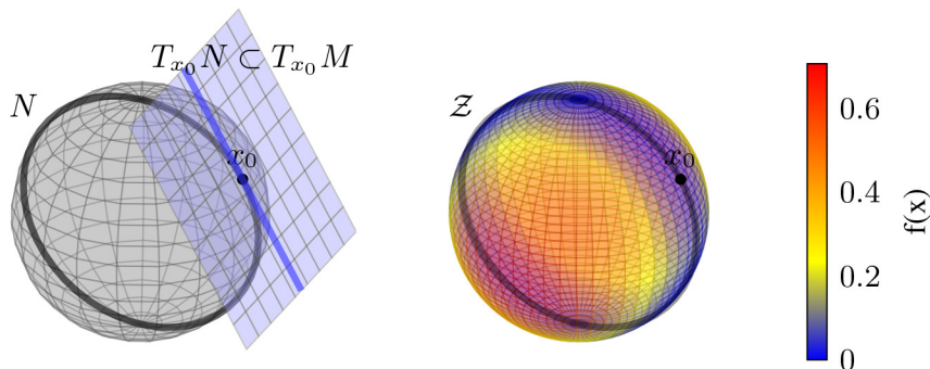
FIG. 6. Left: Representation of the manifold M = S^2 as well as a submanifold N homeomorphic to a circle. The tangent spaces at a given point x_0 \in N \subset M are represented as well. Right: Representation of a nonnegative function on the sphere as a color map; it satisfies the NHC, and its null space \mathcal{Z} is represented in black. (Note that color appears only in the online article.)
