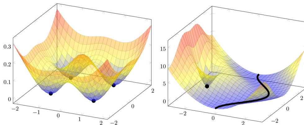
FIG. 1. Plots of functions z = f(x, y) , where the zeros of f are highlighted in black. left: f satisfies the SHC, right: f satisfies the normal Hessian condition but not the SHC.
