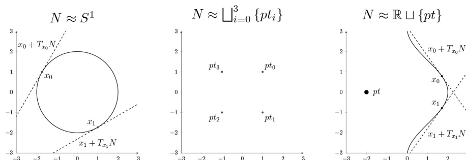
FIG. 2. Examples of submanifolds of \mathbb{R}^2 ; points are denoted with pt . Left: connected submanifold of dimension 1 (a circle). Center: a submanifold of 4 connected components which are all points, i.e., of dimension 0 (their tangent space is not represented since it is reduced to \{0\} ). Right: a submanifold of two connected components, one point pt of dimension 0 and one of dimension 1.
