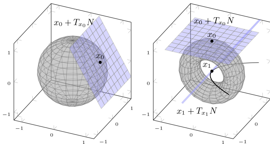
FIG. 3. Two examples of submanifolds of \mathbb{R}^3 . The blue affine spaces represent tangent spaces. Left: connected submanifold of dimension 2 (the sphere S^1 ). Right: a submanifold of two connected components, one of dimension 2 (homeomorphic to the torus \mathbb{T}^2 on which lies x_0 ), and one of dimension 1 on which lies x_1 .
