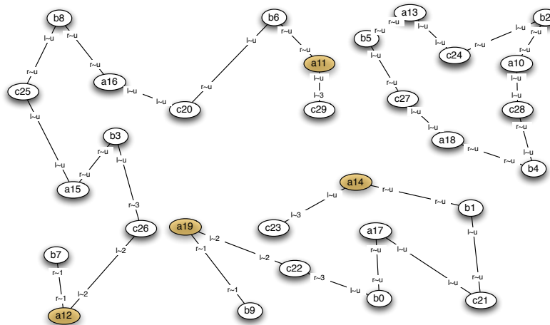
Figure 5: The ambiguity of the lc rules, in the absence of group names, is causing other shapes than the expected triangles to appear. The particular state presented above was obtained by a stochastic simulation starting with 10 of each agents. A 9-gone has formed already, but the the remaining chains are still active, and with probability will eventually loop. Note also that the only remaining active agents of type a are the chain ends.
